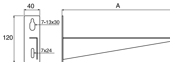
B9/75-320
